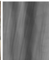
Storm Cloud
